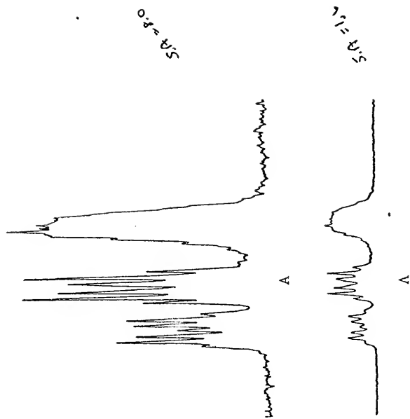
Figure 9 - ^{19}\text{F} NMR of \text{CF}_2\text{BrCFClCH}_2\overset{\text{A}}{\text{C}}\text{HCH}_2\overset{\text{A}}{\text{C}}\text{HBrCF}_3
